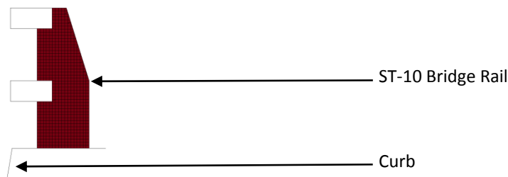
Figure 10-15 Fully Constrained Test Article
