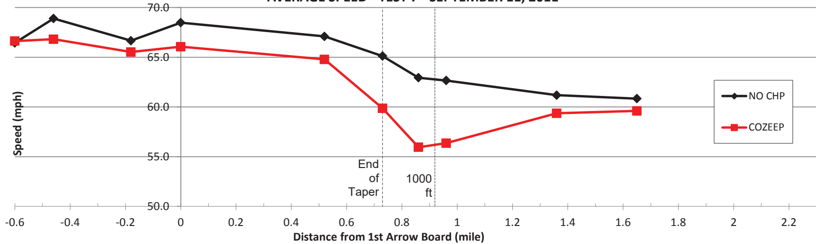
AVERAGE SPEED - TEST 7 - SEPTEMBER 11, 2011
