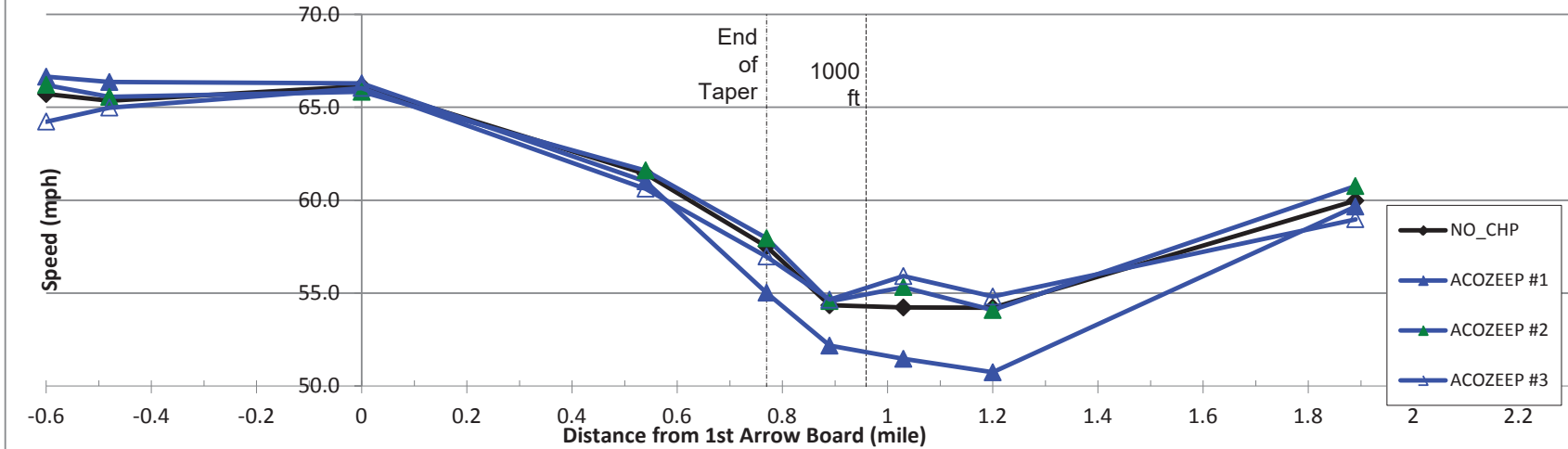
AVERAGE SPEED - TEST 8 - SEPTEMBER 12, 2011
