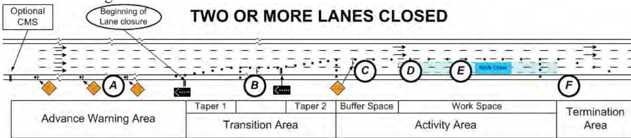
Figure 8. A Sample Work Zone Layout with two-lane Closure
