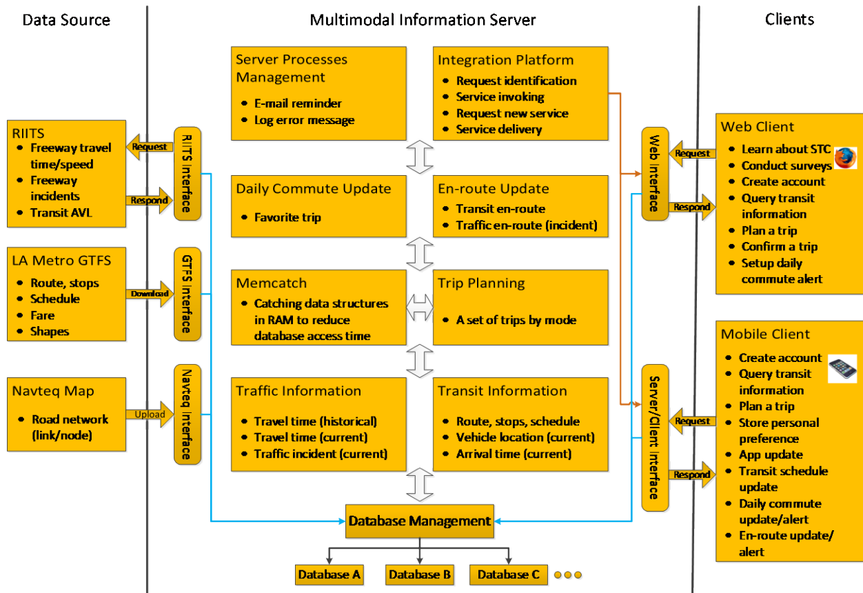
Figure 2-1 Trip2go Architecture
