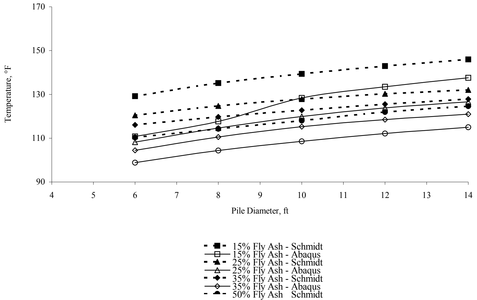
Figure 3-59 - Maximum Temperature – Schmidt versus ABAQUS – Series 2 - (Total Cementitious Materials 591 lb/cy)
