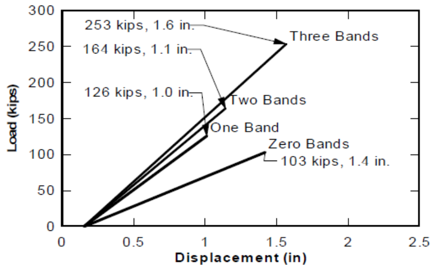
Load Displacement for Zero, One, Two, and Three Band Sand-Jacks
