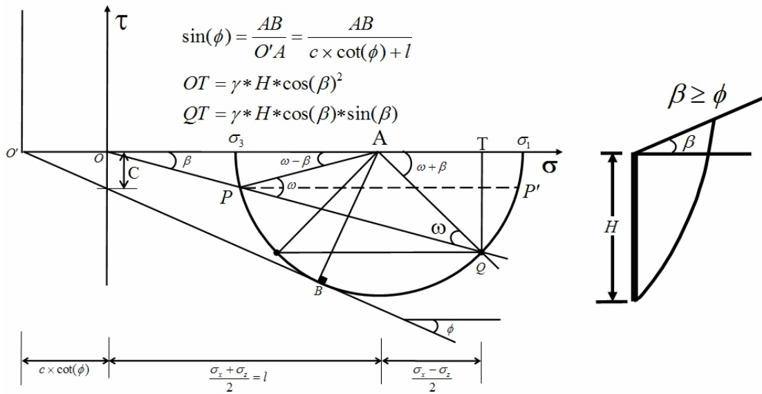
Figure 4-13. Sloping Ground
