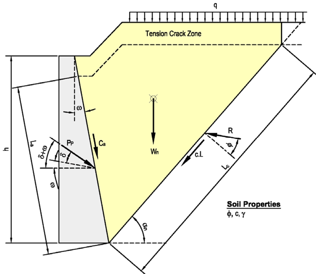
Figure 4-15. Passive Trial Wedge
