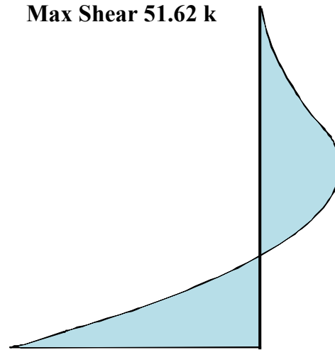
Figure 6-26. Shear Diagram
